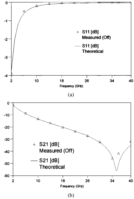
Fig. 8. Return loss and insertion loss for the "off" state: comparison between: (a) theoretical and (b) experimental data [13].
