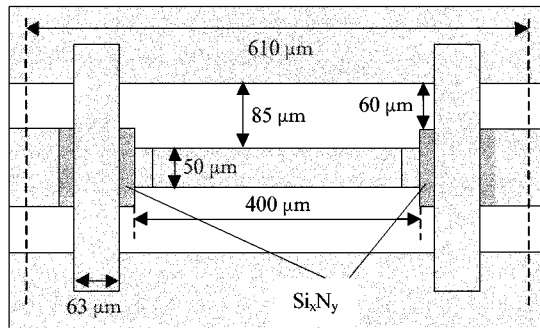
Fig. 12. Double switch [16]: two switches are connected by a 400- \mu\text{m} -long high-impedance line in order to reduce return loss in "on" state while obtaining high insulation in the "off" state.
